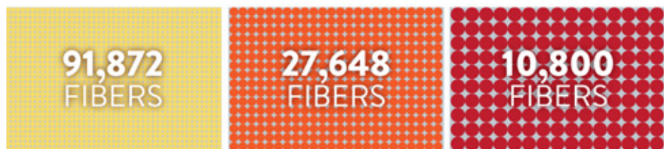
72-Fiber Rollable Ribbon Cable 12x8" Ladder Rack - 44x29 72-Fiber Flat Ribbon Cable 12x8" Ladder Rack - 24x16 72-Fiber Tight Buffered Cable 12x8" Ladder Rack - 15x10
