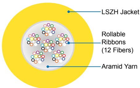
72-Fiber R-Pack Rollable Ribbon LSZH Dual Rated Backbone Cable Cross-Section
