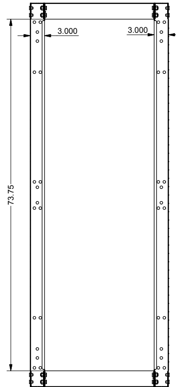
SECTION B-B
