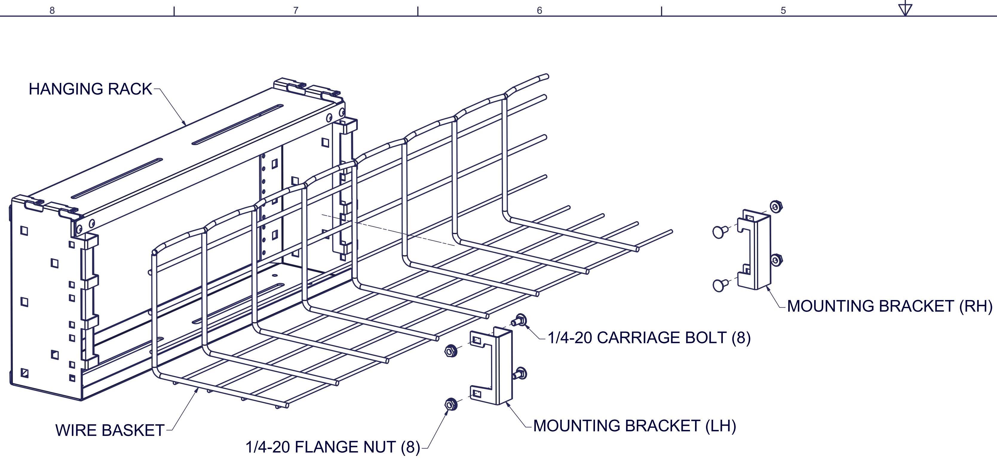
REAR EXPLODED VIEW
