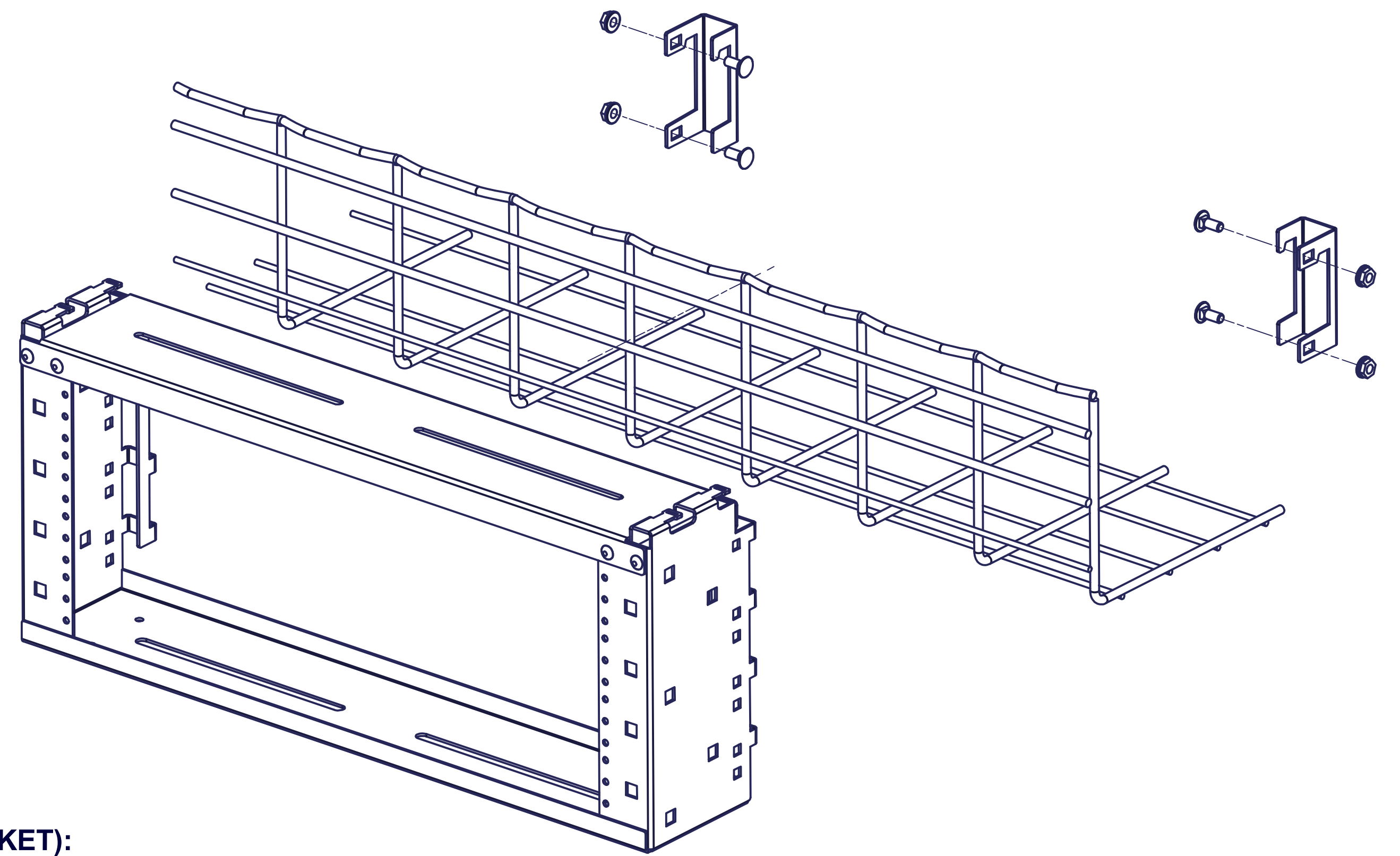
FRONT EXPLODED VIEW
