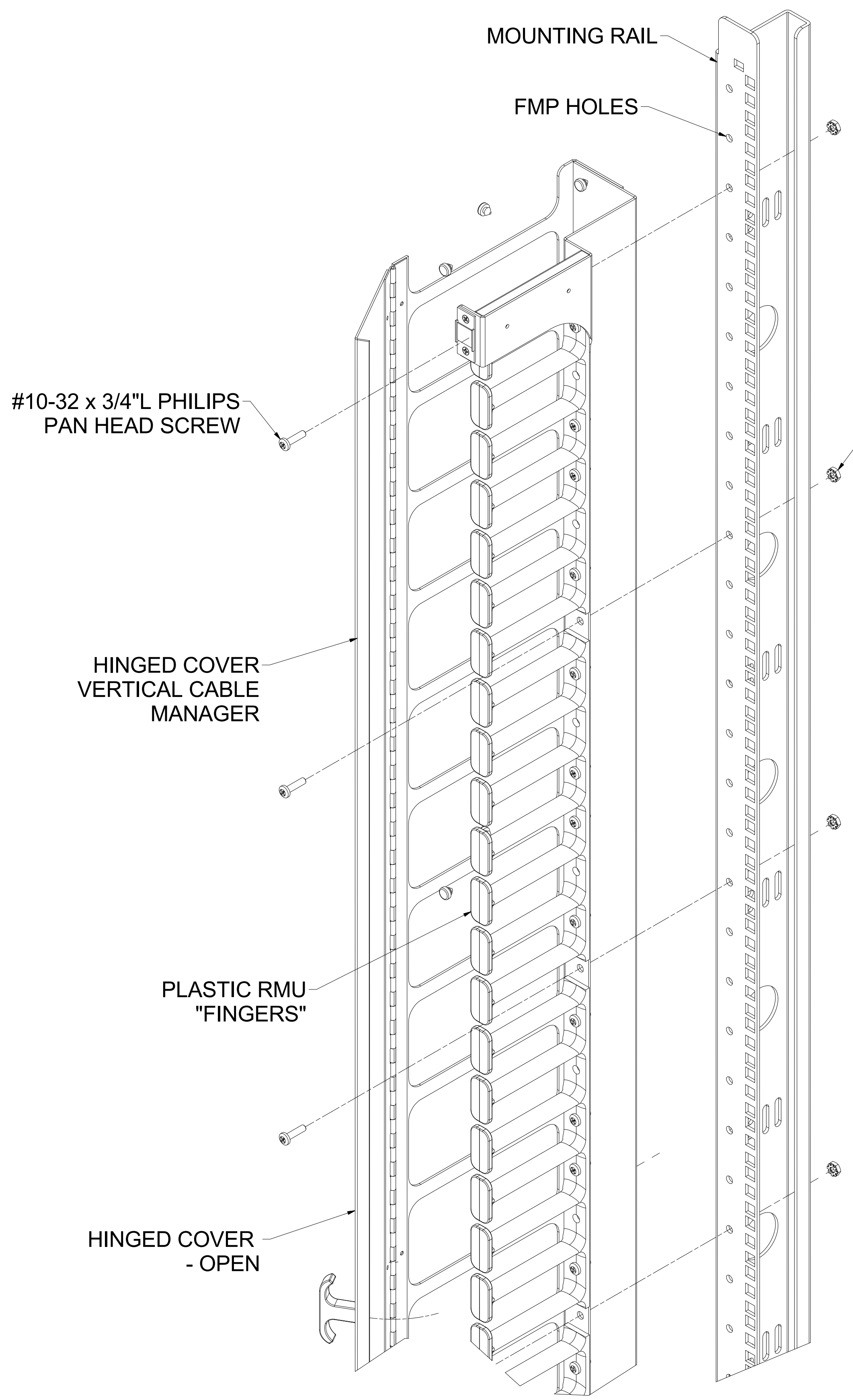
DETAIL N
