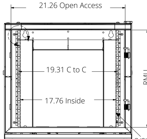
FRONT VIEW WITHOUT DOOR
