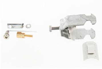
FIST® GR2/3 Outer C-cable clamp, for 1 cable with 22-28mm diameter, 1 pce
