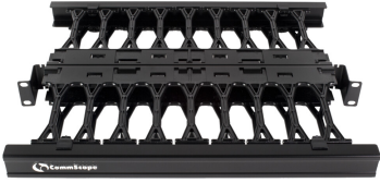
Horizontal Trough Kit, 19 in rack mountable, double sided, 1 RU
