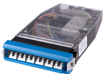
G2 Splice Cassette, 12LC/UPC with internal shutters, OS2, with 250 μm pigtails
